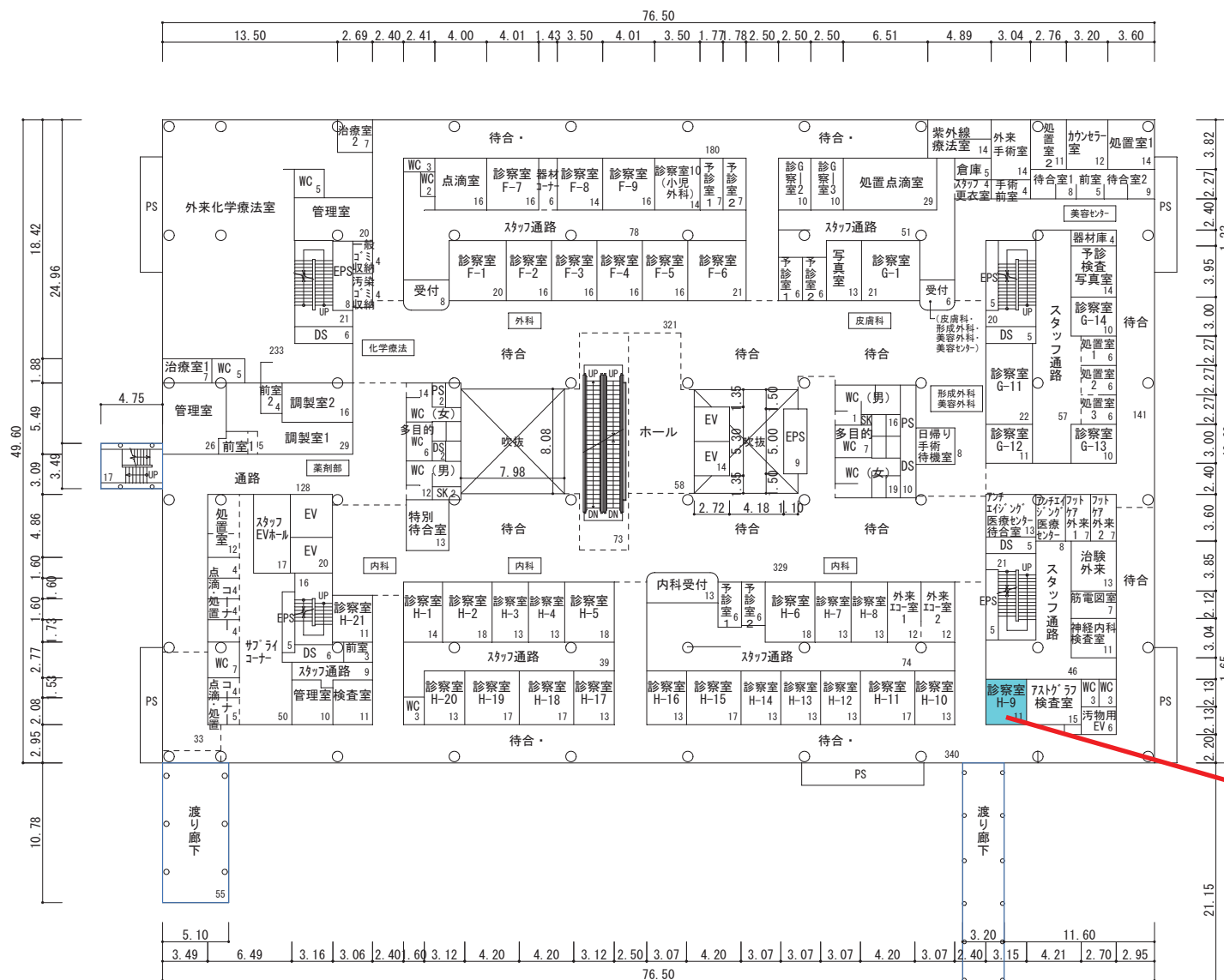
3 階平面図・ s = 1 / 500 (3,825m 2 )
